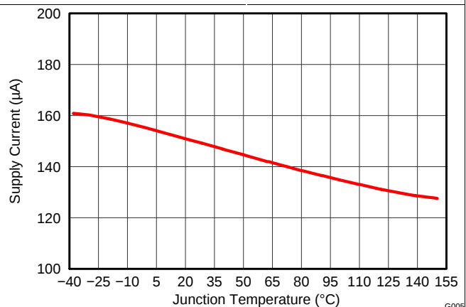
Figure 6. Input Voltage Quiescent Current vs. Temperature
