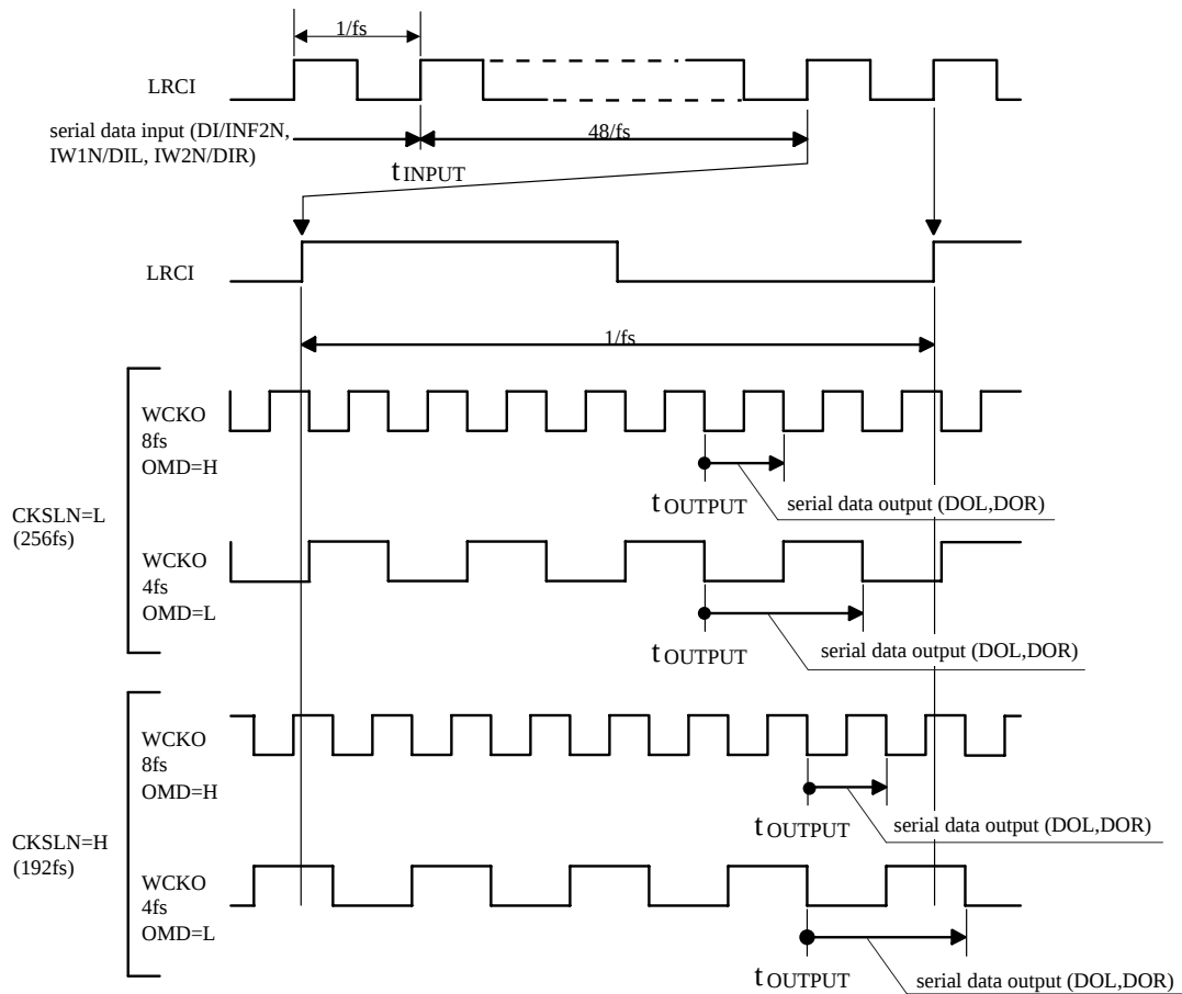
Figure 6. Group delay timing (SYNCH = LOW)
