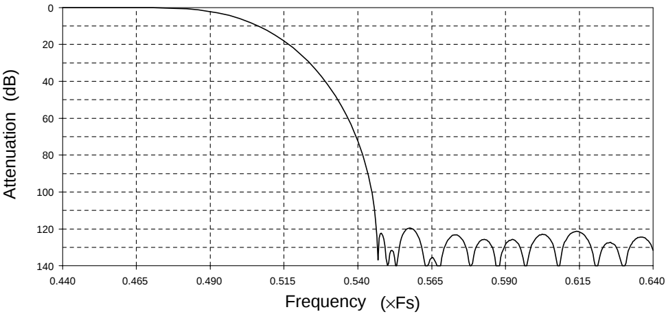
8fs filter transition response with deemphasis OFF
