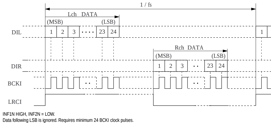
Figure 5. LR alternating, leading data, 24-bit input
