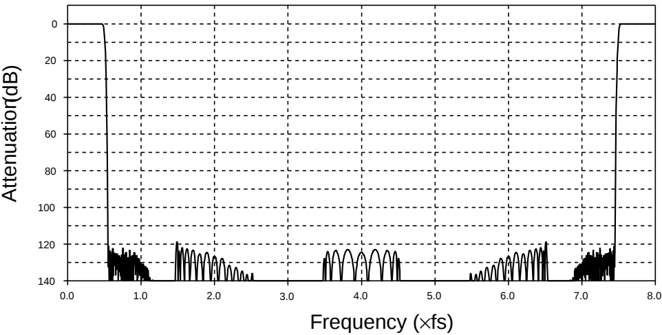
8fs filter passband response with deemphasis OFF
