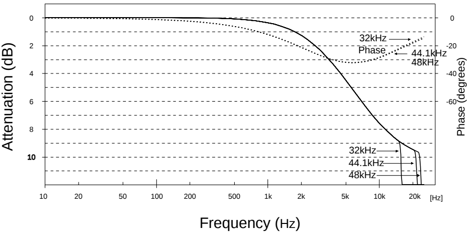
Passband response with deemphasis ON (logarithmic frequency axis)
