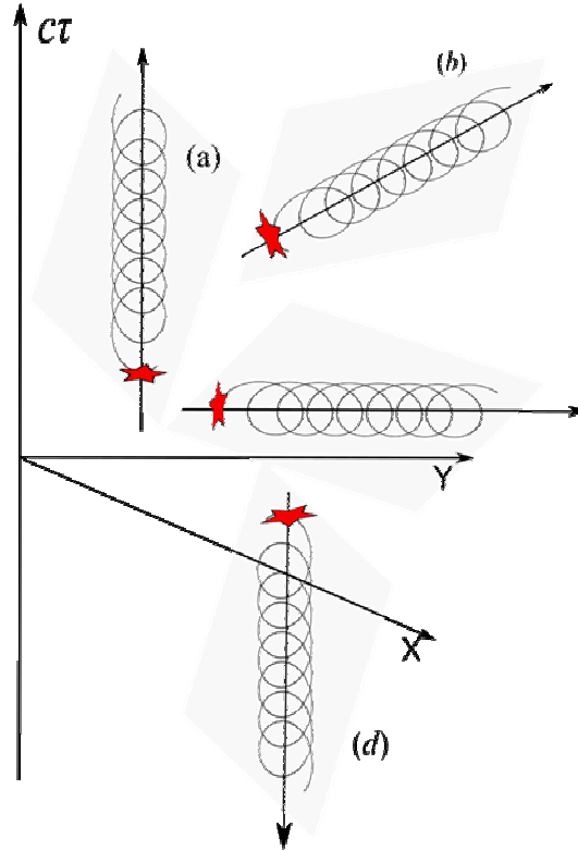
Figure 1. A few examples of particles creation (a) – a T-particle at 3D absolute rest moves along ct -axis; (b) – a T-particle moves also in 3D space; (c) – a photon moves only in 3D space; (d) – a T-antiparticle moves along ct -axis in negative direction. Stars point events when an lattice FLE is impacted. Note that this is only some illustrative picture, in 4D space a 4D T-particles “helices” on Figure don’t exist, so that can be quite equally painted relatively to (X,Z) and (Y,Z) planes as well.
