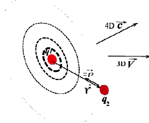
Figure 7 A sketch of a spreading of the circular photons in the 3D space that are radiated by moving particle. The directions of the spreading rims' planes are random in 4\pi , since any particle in a body is impacted by some forces, however unlike the absolute rest case above all T-particles in moving body at 3D space motion have the same additional caused by impacting 3D momentum precessing, and so all are oriented also in the 4D and 3D spaces.
