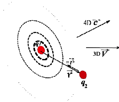
Figure 7 A sketch of a spreading of the circular photons in the 3D space that are radiated by moving particle. The directions of the spreading rims' planes are random in 4\pi , since any particle in a body is impacted by some forces, however unlike the absolute rest case above all T-particles in moving body at 3D space motion have the same additional caused by impacting 3D momentum precessing, and so all are oriented also in the 4D and 3D spaces.
